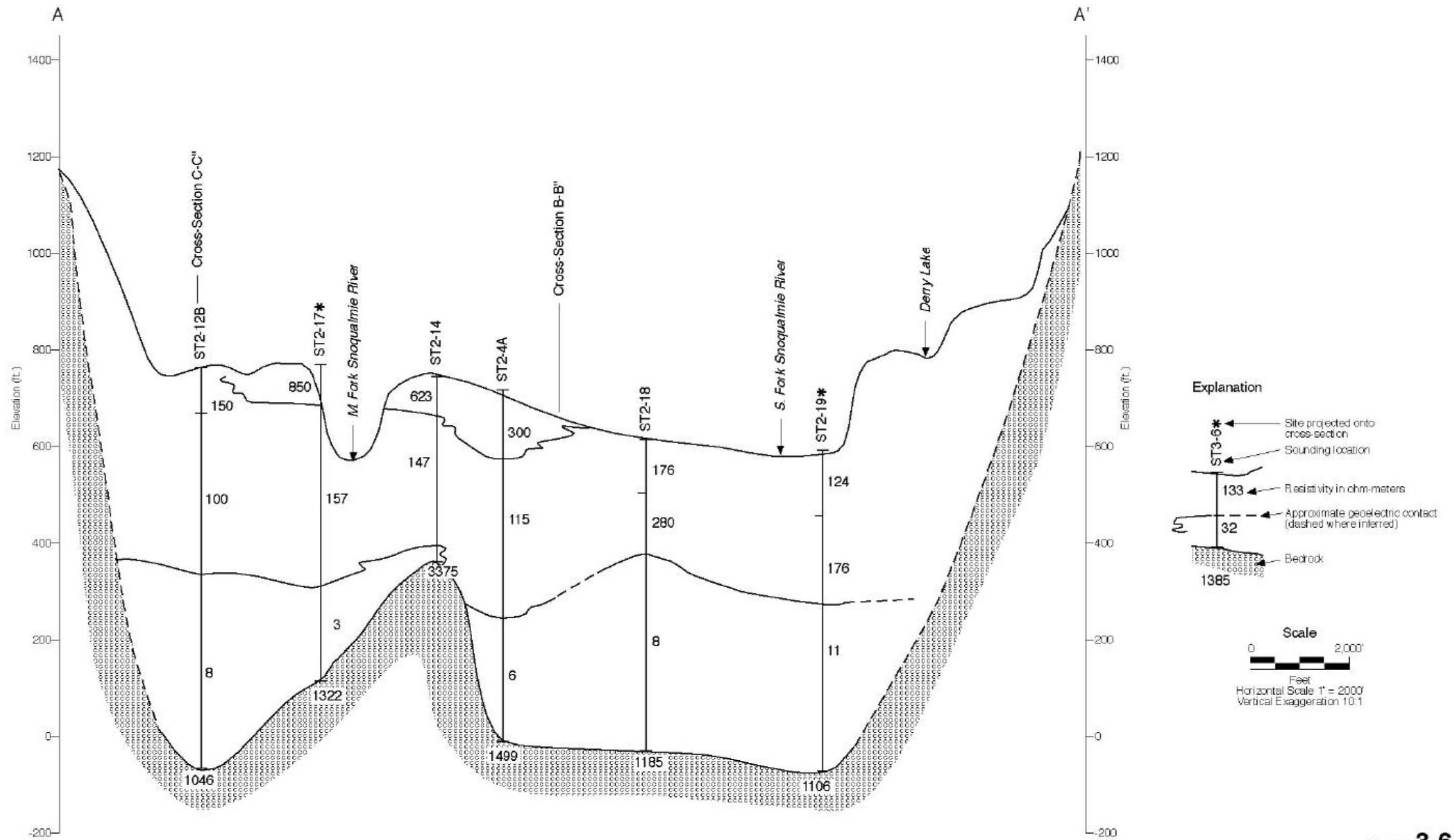
FIGURE 3-6 GEOELECTRIC CROSS-SECTION A-A' AREA 2 EKRWA/WATER SUPPLY/WA
