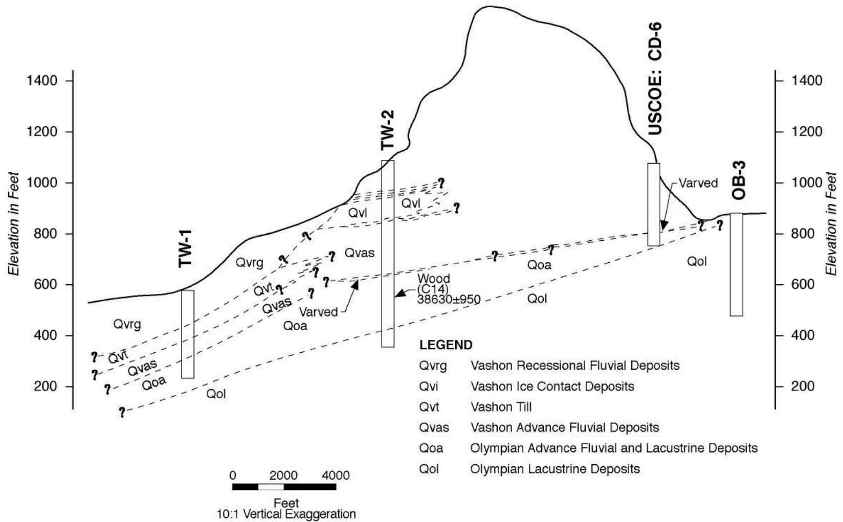
FIGURE 2 GENERALIZED GEOLOGIC CROSS SECTION EKCRWA/WATER SUPPLY/WA
