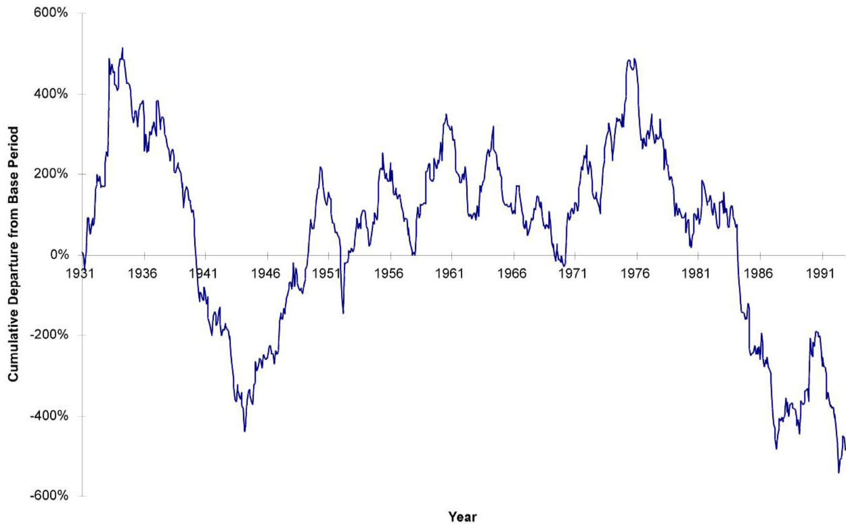
FIGURE 3-1 LONG TERM VARIATIONS IN PRECIPITATION AT CEDAR FALLS EAST KING COUNTY/WATER SUPPLY/WA
