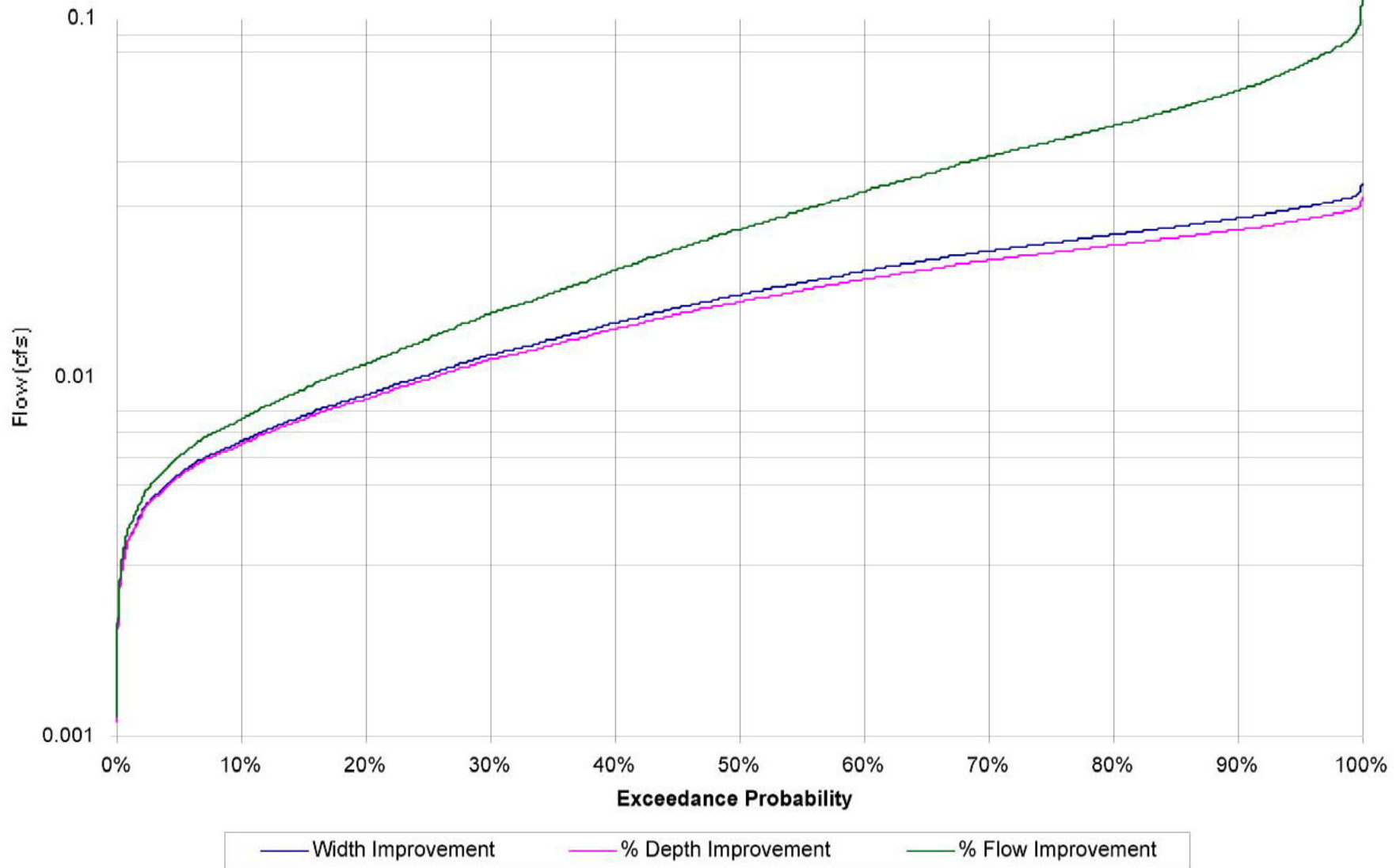
FIGURE 5-1 PREDICTED IMPROVEMENT IN FLOW AND WATER DEPTH AT CARNATION FROM AUGMENTATION WITH 40 CFS EAST KING COUNTY/WATER SUPPLY/WA
